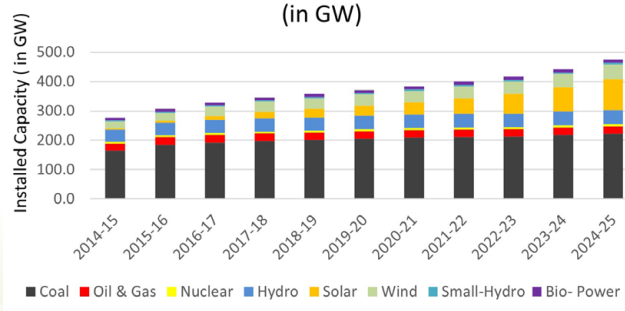
Source-wise Electricity Installed Capacity Trends from 2014-15 to 2024-25 (as on 31.03.2025) (in GW)
