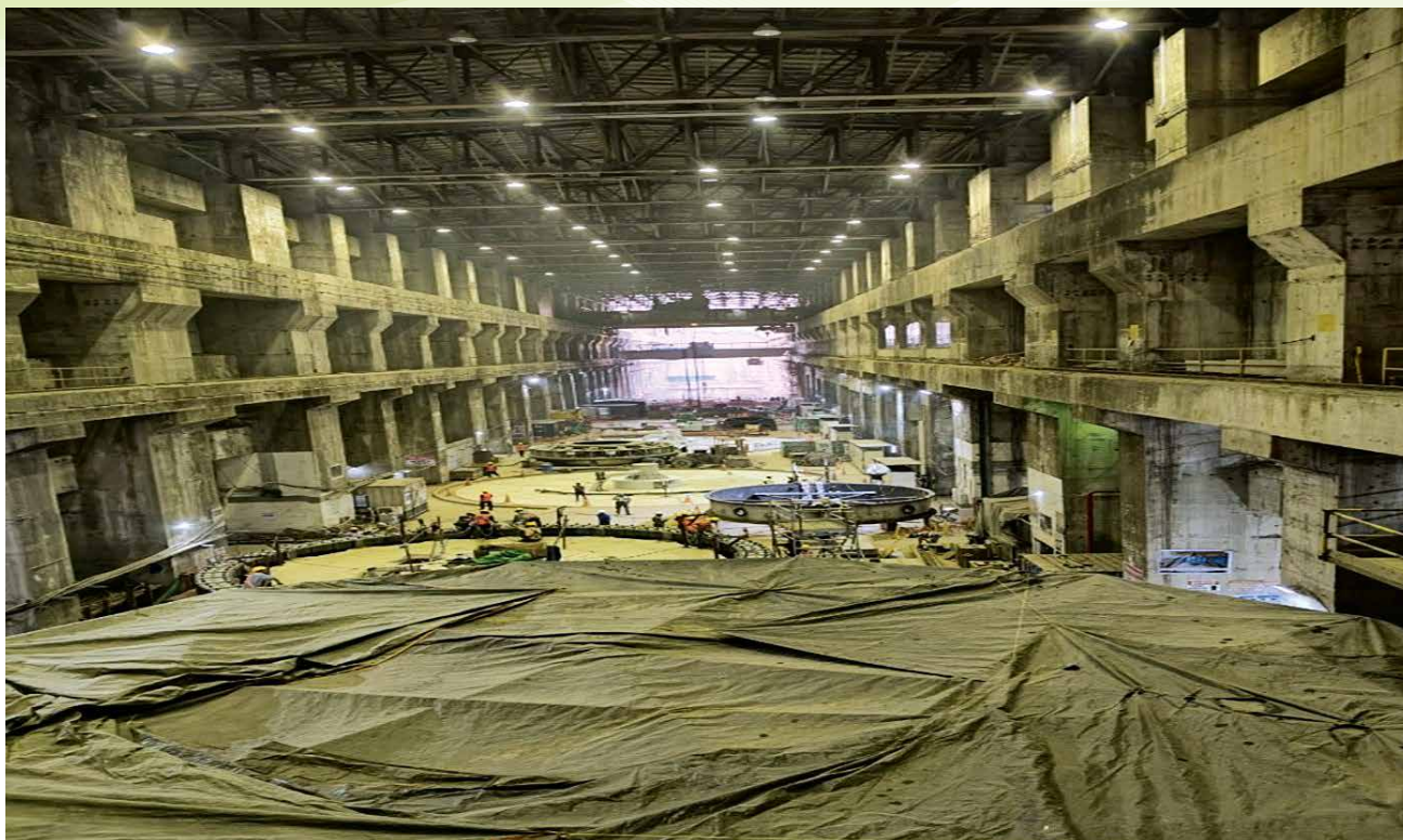
VIEW OF POWER HOUSE FROM UNIT-1 SIDE – 2000 MW SUBANSIRI LOWER PROJECT (ARUNACHAL PRADESH)
