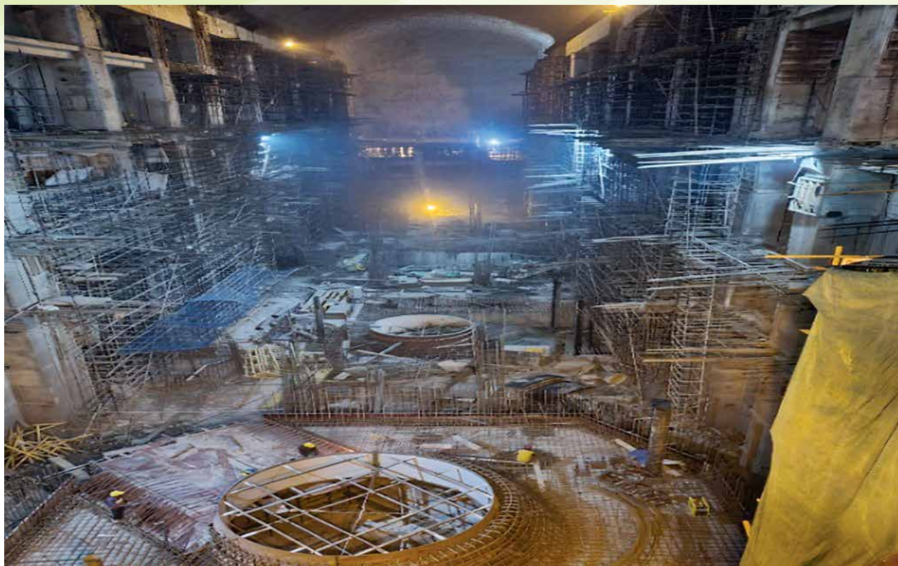
POWER HOUSE- 624 MW KIRU PROJECT (UT OF J&amp;K)
