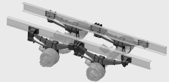
Sleeper Suspension
