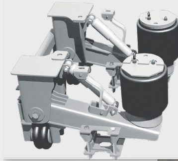
Trailer Air Suspension
