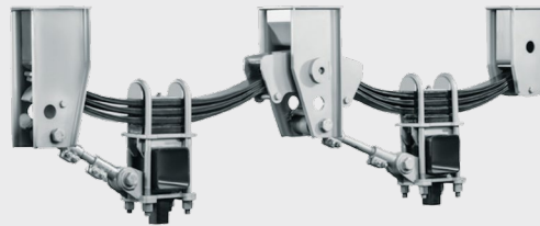
Trailer Mechanical Suspension
