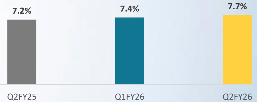
PAT Margins (%)
