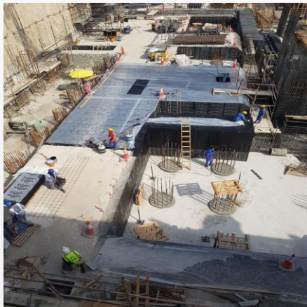
De-watering Project at One Za'abeel Tower, Dubai
