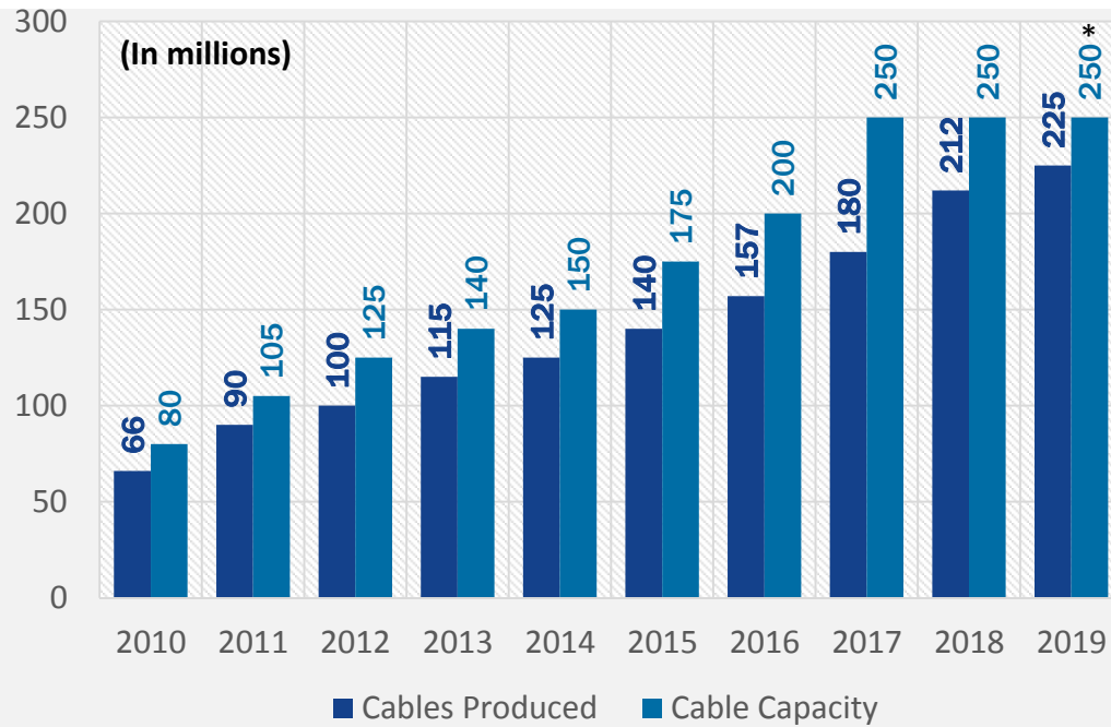
Cable Capacity
