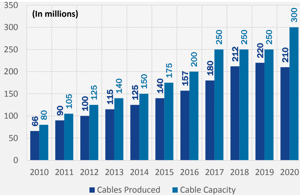
Cable Capacity
