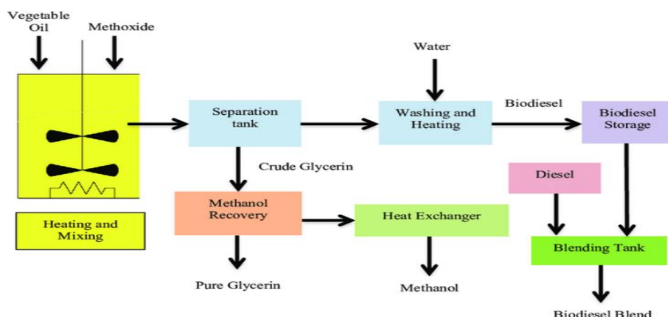
Figure 37: Biodiesel process flow
