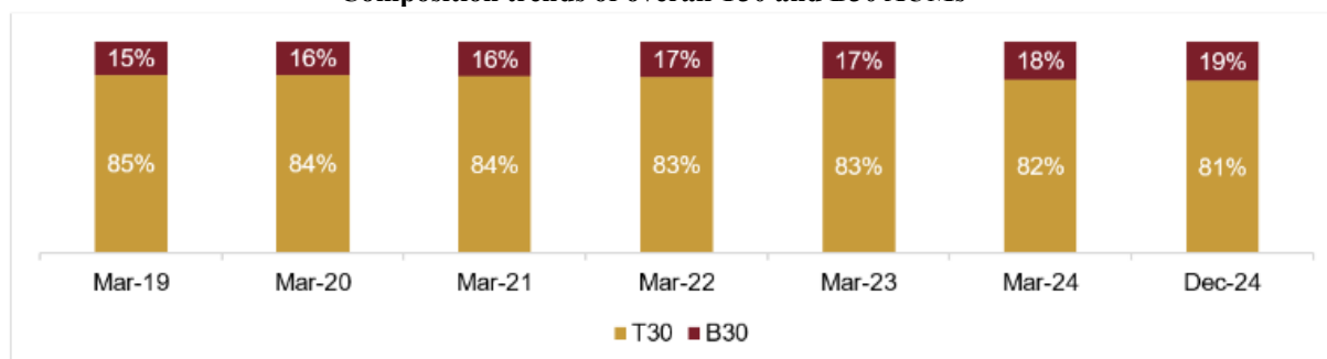
Composition trends of overall T30 and B30 AUMs
